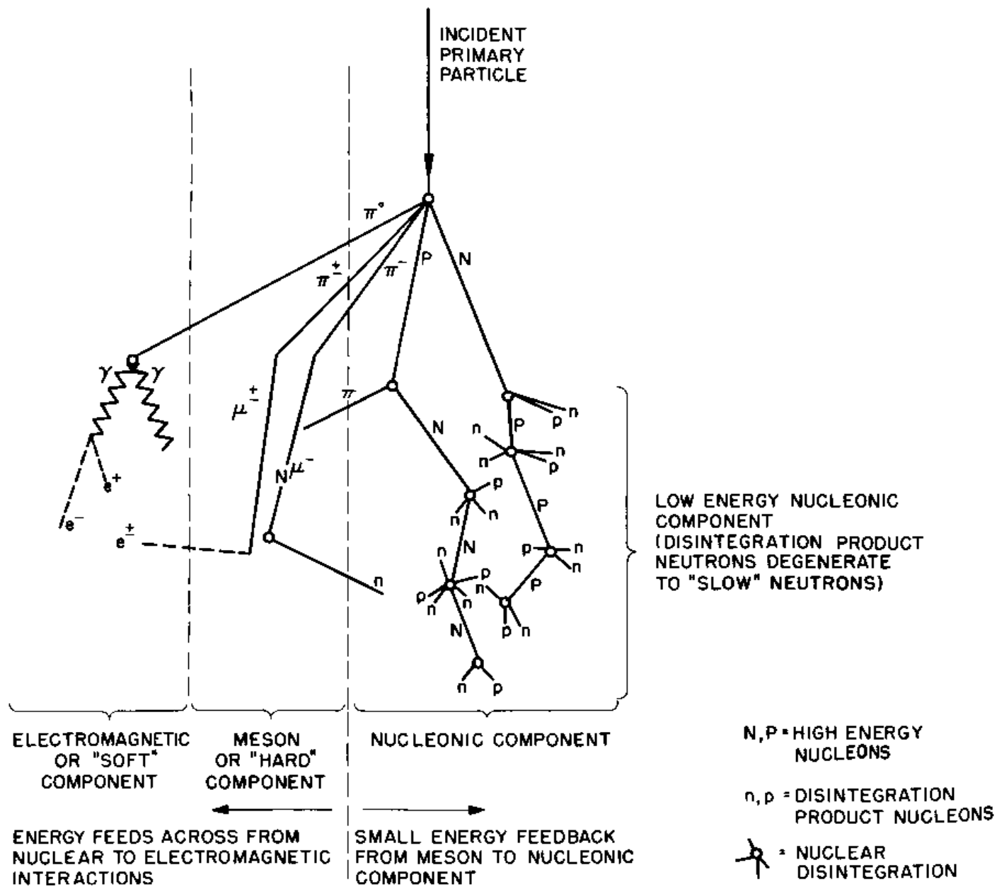
Schematic Diagram of Cosmic Ray Shower
